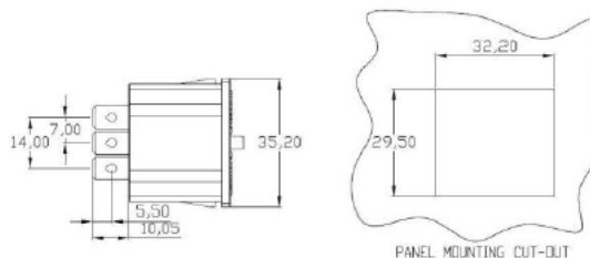
PANEL MOUNTING CUT-OUT
